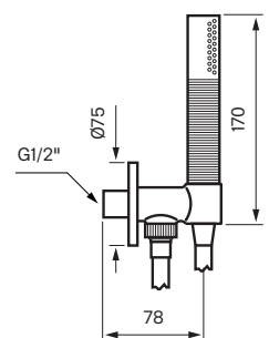
Hand shower
